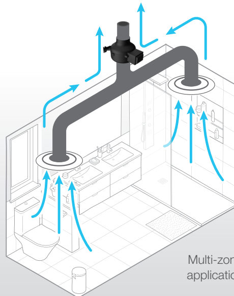
Single zone application
